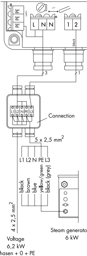
Connection plan 6 kW
