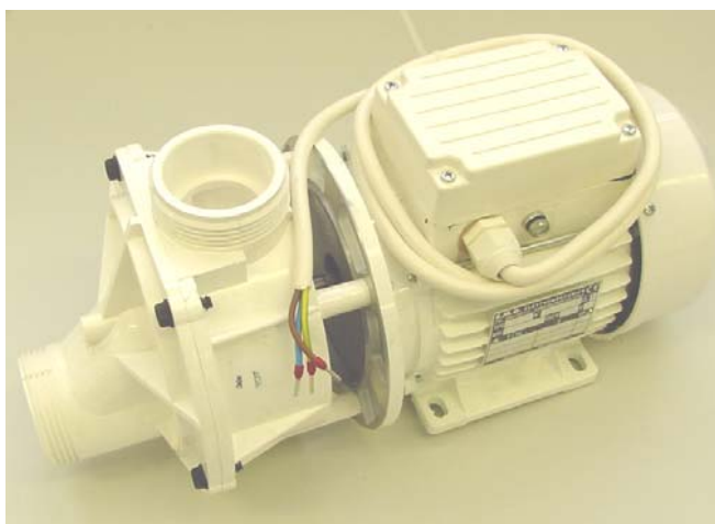
Hydropumpe 21802000
