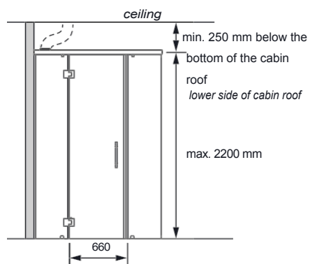
INSTALLATION EXAMPLE: CABIN ROOF CONNECTED TO GLASS FRONT.
