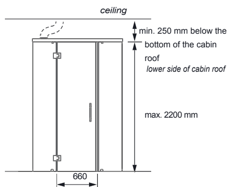
INSTALLATION EXAMPLE: CABIN ROOF CONNECTED TO GLASS FRONT.
