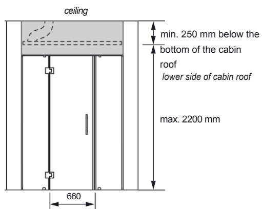
INSTALLATION EXAMPLE: BUILT-IN CABIN ROOF.
