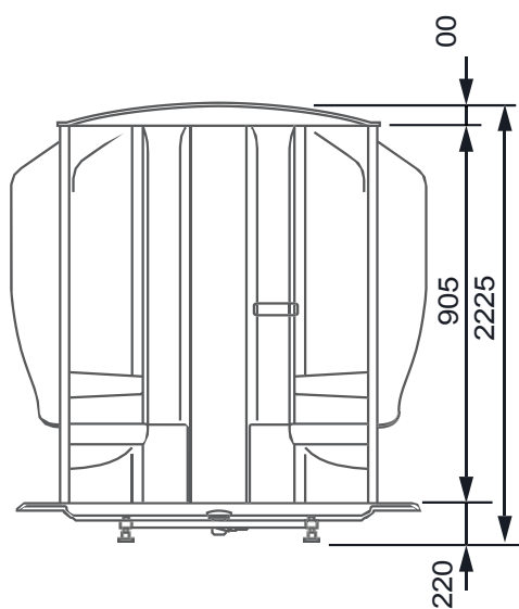
Front view (in mm)
